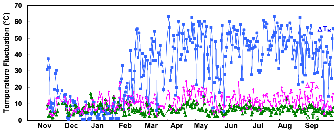
Figure 4.13: The daily ambient temperature ( T_A ) fluctuation and temperature fluctuations on the Reference ( T_R ) and Green ( T_G ) roof membranes (November 2000 to September 2001).
