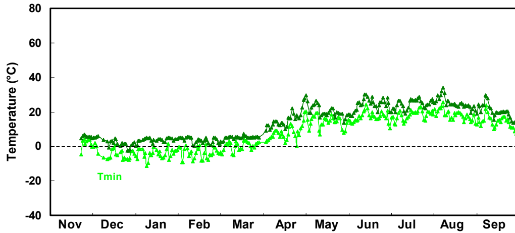
Rooftop Garden - Membrane Temperature (Nov 22, 2000 - Sep 31, 2001)
