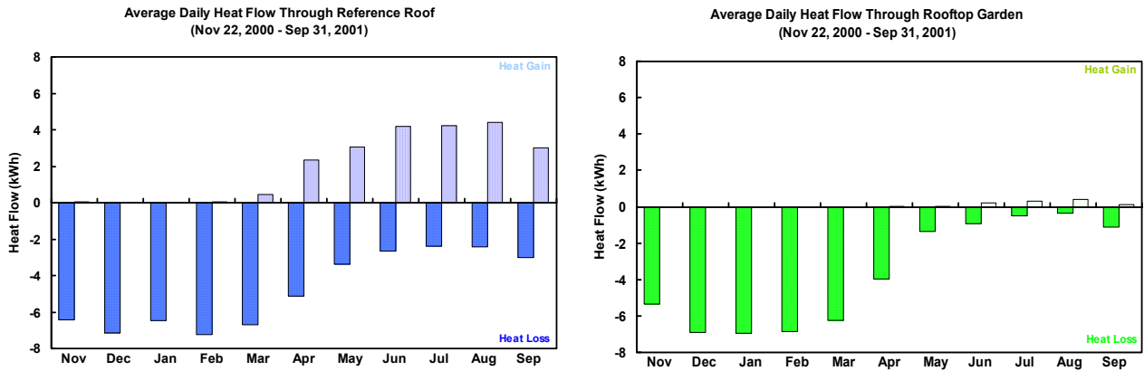
Figure 4.21: Average daily heat flow through Reference and Green Roofs (kWh)
